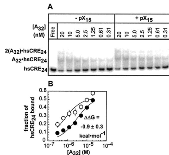
FIGURE 8: Influence of pX 15 on the equilibrium stability of a bZIP monomer-DNA half-site complex. (A) Gel representative of the equilibrium binding of A 32 to hsCRE 24 in the presence (lanes 9–15) and absence (lanes 2–8) of 20 μM pX 15 . Due to the high peptide concentrations that are necessary to detect monomer binding, it is likely that the second shift that is visible on the gel is due to nonspecific second site binding. (B) Quantitative electrophoretic mobility shift analysis of A 32 ·hsCRE 24 complexation in the presence (○) or absence (●) of 20 μM pX 15 at 25 °C. K_d(-\text{pX}_{15}) = (3.1 \pm 0.7) \times 10^{-6} \text{ M} , and K_d(+\text{pX}_{15}) = (7.0 \pm 2.2) \times 10^{-7} \text{ M} .
